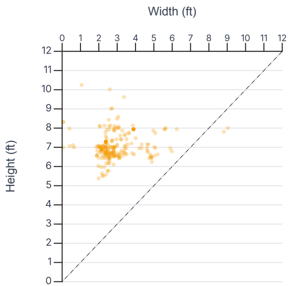
Opening Aspect Ratio
